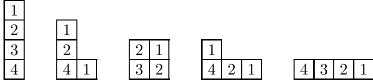
Fig. 1.4. The multi-set of hook lengths for \mathcal{P}(4)
